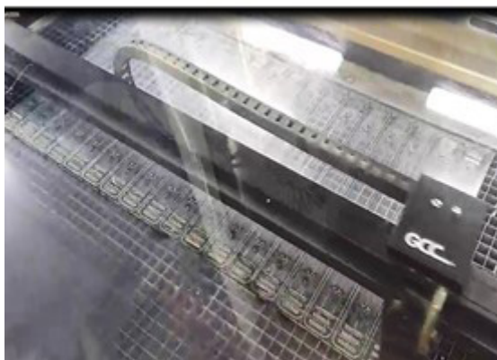
Figure 5. Devised full face transparent shield – stages of fabrication a) ready product; b) pattern for laser cutting; c) laser cutting of forehead strip
