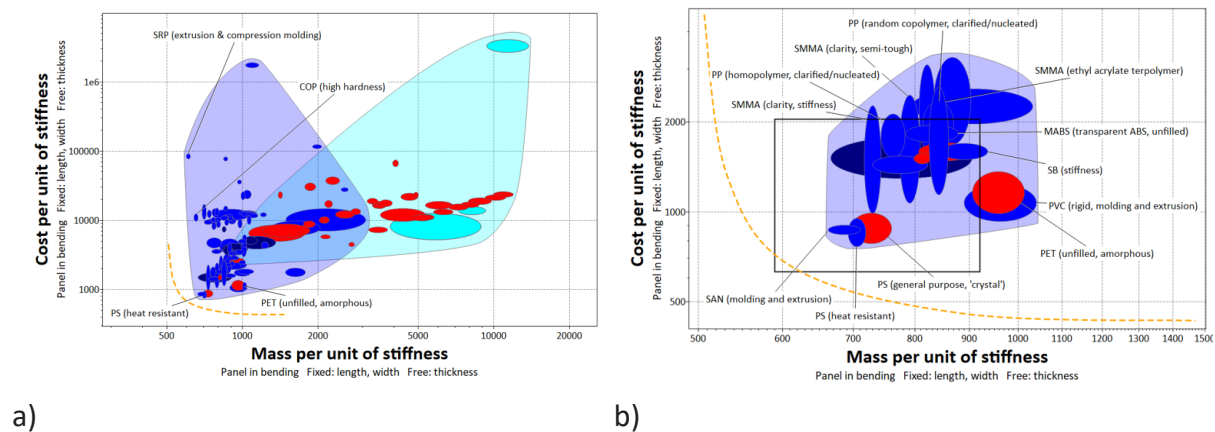
Figure 4. Material selection for transparent medical face masks. Ranking stage: a) 129 candidates; b) 19 candidates (red - optical quality; blue – transparent), [7].
